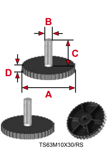
TS63M10X30/RS
