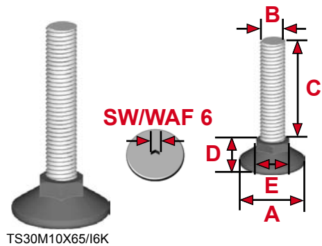
TS30M10X65/I6K
